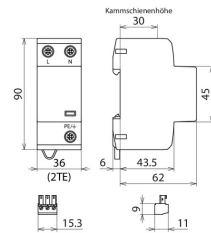
Dimension drawing DSH TT 2P 255 FM
